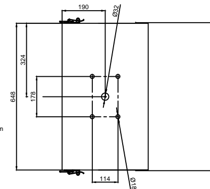
Mounting holes punched in top and bottom of the case. Scale 1:2
